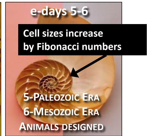
Nautilus Shell
