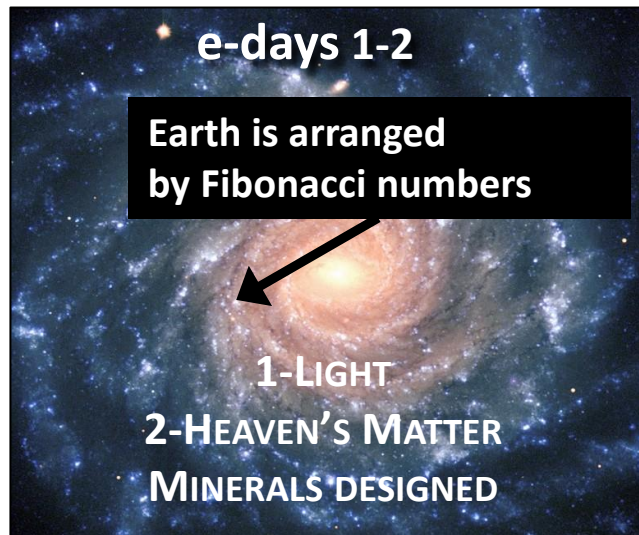
Galaxy
