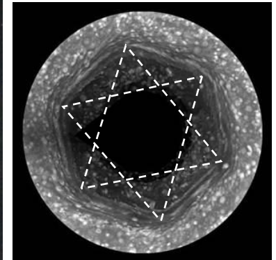
Polar cloud
